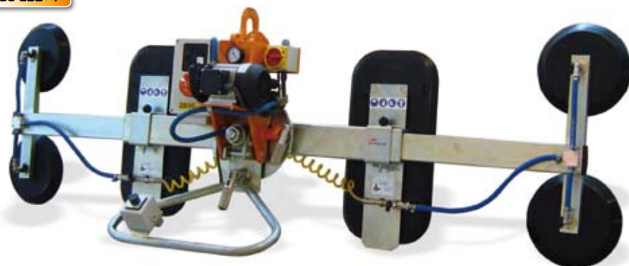
VX30-GB2+4
