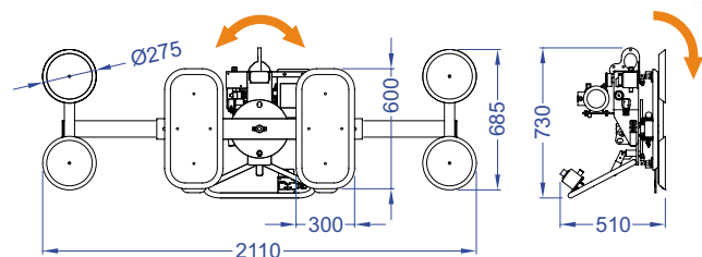
VX30-GB2
